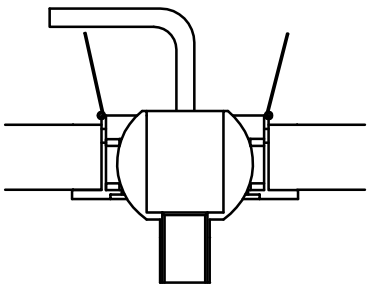
(2) Bend back springs and push into cut out hole.
