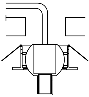
(1) Gently hold fibre optic tail in one hand and screw fitting onto ferrule as far as it will go.
