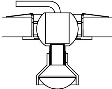
(4) A narrow beam of light is produced when the trumpet is screwed on with a few threads.
