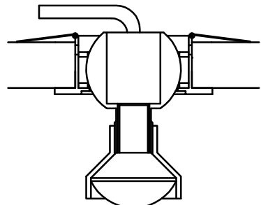
(3) Screw trumpet onto fitting.
