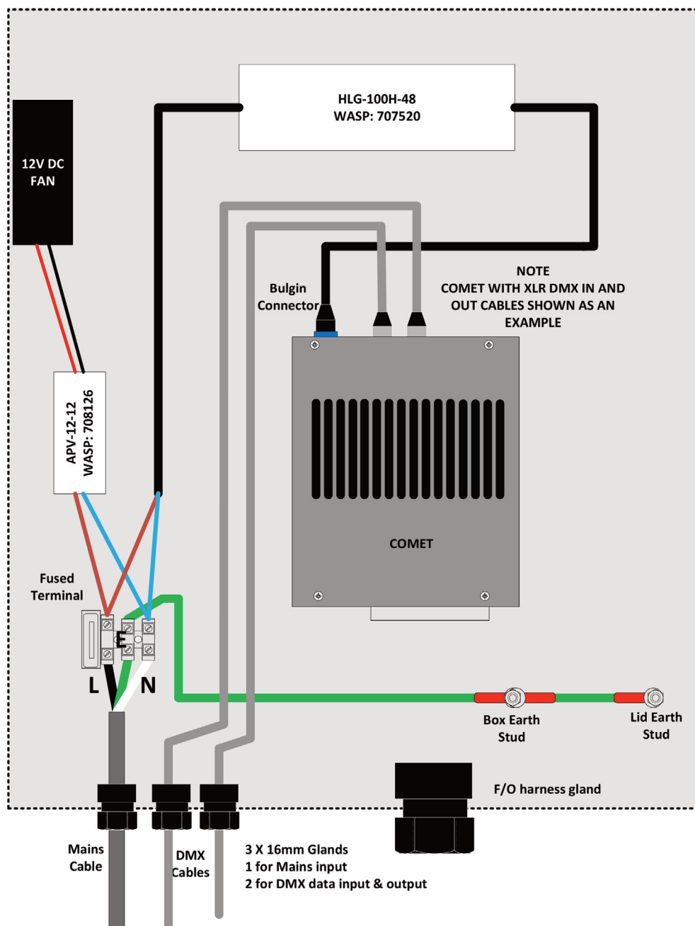
FIGURE 1 - AC SCHEMATIC USING COMET LIGHT SOURCE
