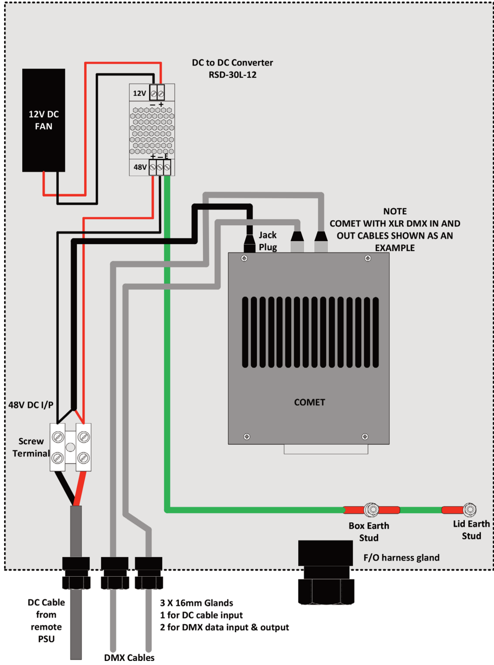
FIGURE 2 - 24V DC SCHEMATIC USING COMET LIGHT SOURCE
